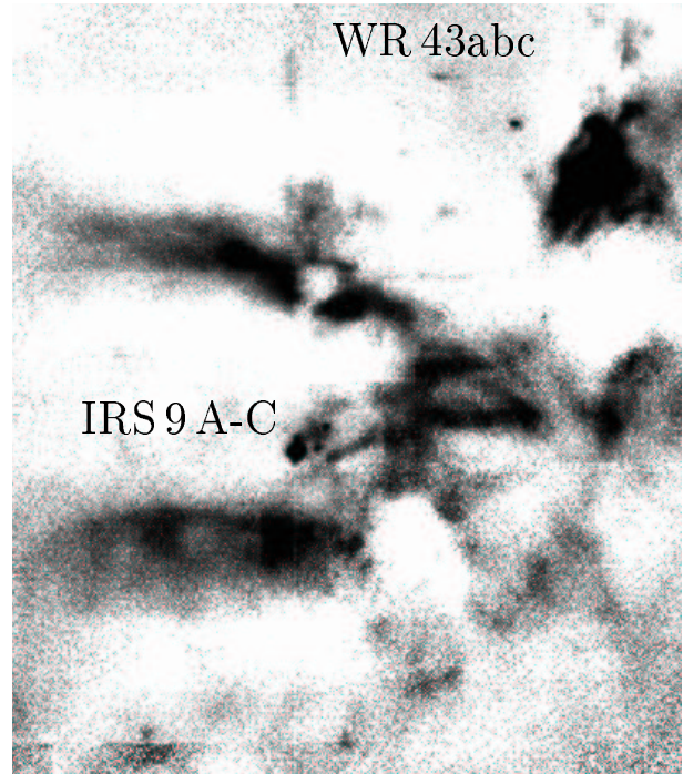
Fig. 1. Central part (FOV = 2'.0 \times 2'.3 ) of our 11.9\ \mu\text{m} NGC 3603 data.
