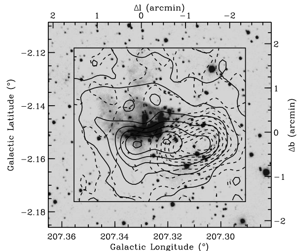
Fig. 1. Integrated \text{HCO}^+(1-0) (solid contours) and \text{CS}(2-1) (dashed contours) emission towards Rosette Cluster No. 3. Notice the offset between the emission peaks. The contours run from 0.25 \text{ K km s}^{-1} in 0.75 \text{ K km s}^{-1} steps. The background image is a JHK composite from FLAMINGOS.
