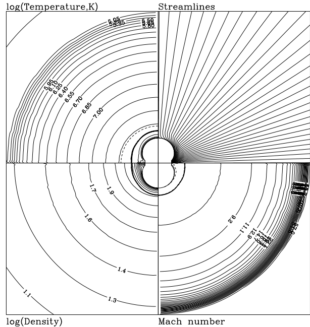
Fig. 1. Accretion pattern stipulated by the radiative cooling and Compton effects.
