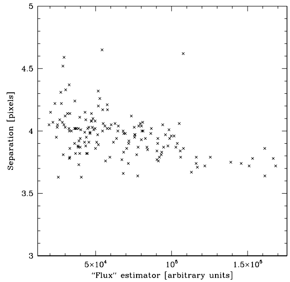
Fig. 4. Mean distance between the three exposures of every star in a frame close to the center of the plate. The instrumental flux provided by SExtractor is employed as an indicator of brightness.
