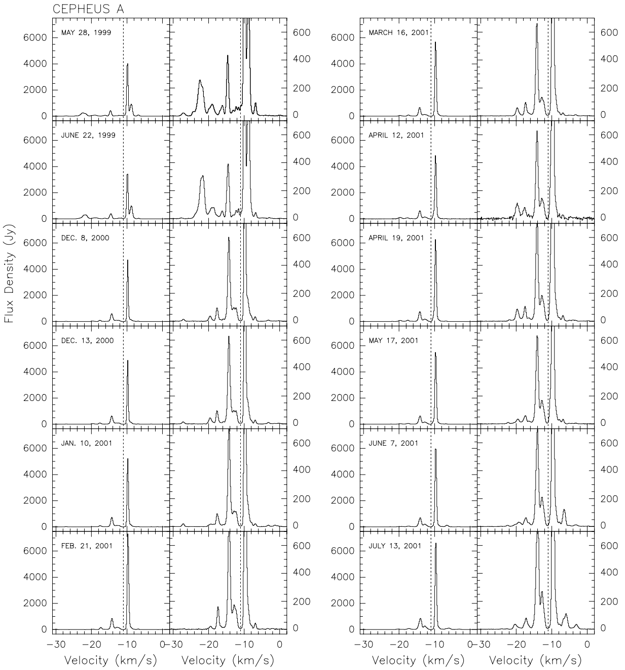
Fig. 10. Same as Fig. 1 but for the Cepheus A source. In this case, the systemic velocity of the source is -11.0 \text{ km s}^{-1} (vertical dashed line). Each spectrum is shown at two different scales to better appreciate the dynamic range of the maser features.
