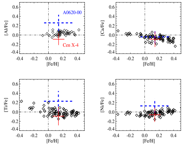
Fig. 1. Abundance ratios of the secondary stars in A0620-00 (thick dashed line cross) and Cen X-4 (thin solid line cross) in comparison with galactic trends
