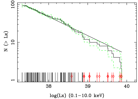
Fig. 2. The XLF of the point-like sources detected in the coadded observation of the Antennae. The straight line show the best fit power-law. The vertical lines in the bottom show the differential XLF, where diamonds indicate sources which appear as ULXs in any of the 7 observations. As in Fig. 1 the band defined by the dashed lines show the typical errors including Poisson uncertainties as well as uncertainties in the source fluxes.
