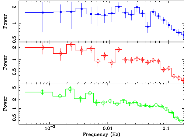
Fig. 1. Power density spectra of the two M31 black hole candidates in M31 in from observations 1, 3 and 4. The left panel shows the PDS of BH1 in observations 1 (top), 3 (middle) and 4 (bottom) with an expected noise level of 0. All three PDS are characteristic of a low accretion rate, even though the luminosity ranges from 1\text{--}3 \times 10^{38} \text{ erg s}^{-1}
