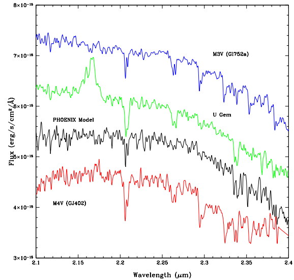
Fig. 1. The infrared spectrum of U Gem (green) compared to those of an M3V (blue) and M4V (red). The black spectrum is a model constructed using the PHOENIX code that has its carbon abundance set to 10^{-2} solar.
