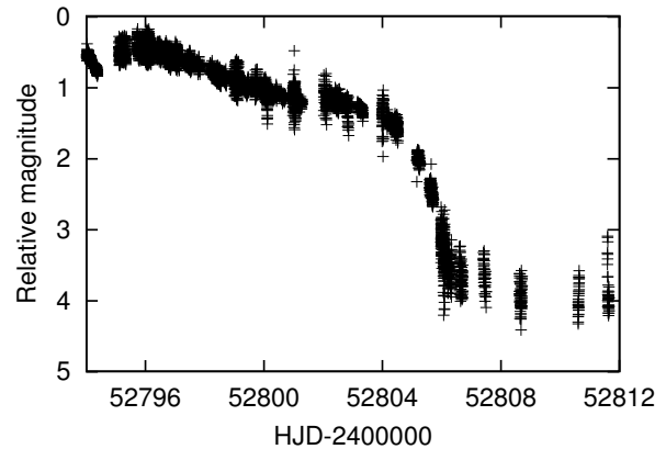
Fig. 1. The light curve of the 2003 superoutburst of GO Com, accompanied with a precursor. The magnitude of the bright maximum corresponds to 13.3 in R. Especially interesting is that the plateau stage lasted for only 8 days.
