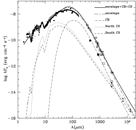
Fig. 1. (Left) Sketch of L1551 IRS5, showing the individual components. (Right) Observed data points (see references in Osorio et al. 2003), and model predicted SEDs for the L1551 IRS5 system.
