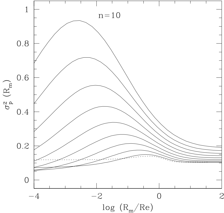
Fig. 5. Plot of the aperture velocity dispersion \sigma_p^2(R_m) , normalized to GM/Re , derived from equation (29) for different values of the exponent n ( n = 1, 2, \dots, 10 ) in the Sérsic profile.
