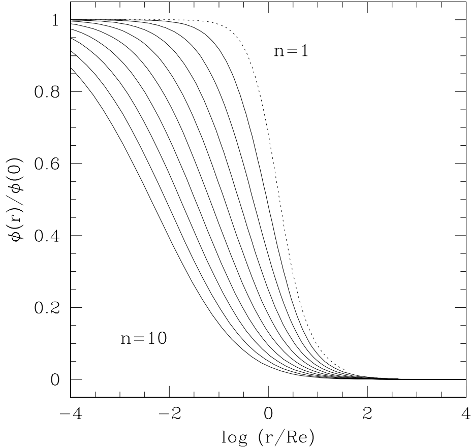
Fig. 3. Curves for the normalized potential \phi(s)/\phi(0) for n = 1, 2, \dots, 10 .
