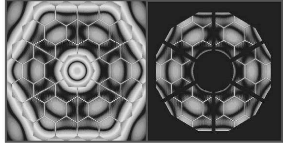
Fig. 4. Left: Pupil image after use of occulting spot at telescope focal plane. Right: Rotating pupil mask applied to pupil image.
