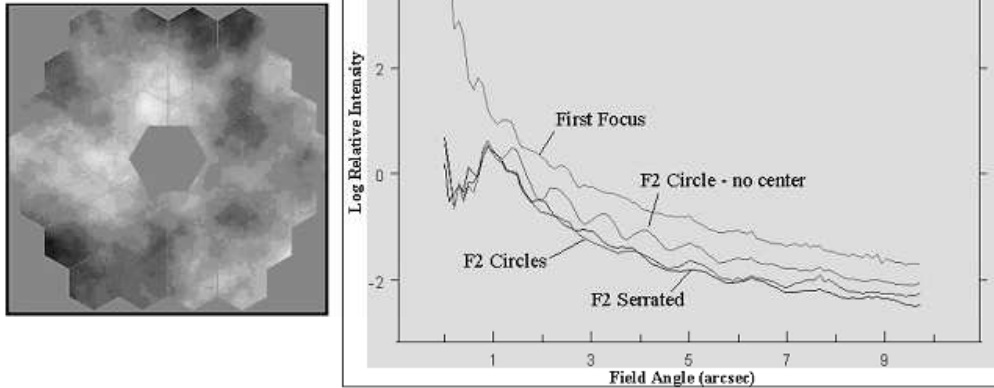
Fig. 3. The telescope pupil. Azimuthal PSF averages with and without the coronagraphic.
