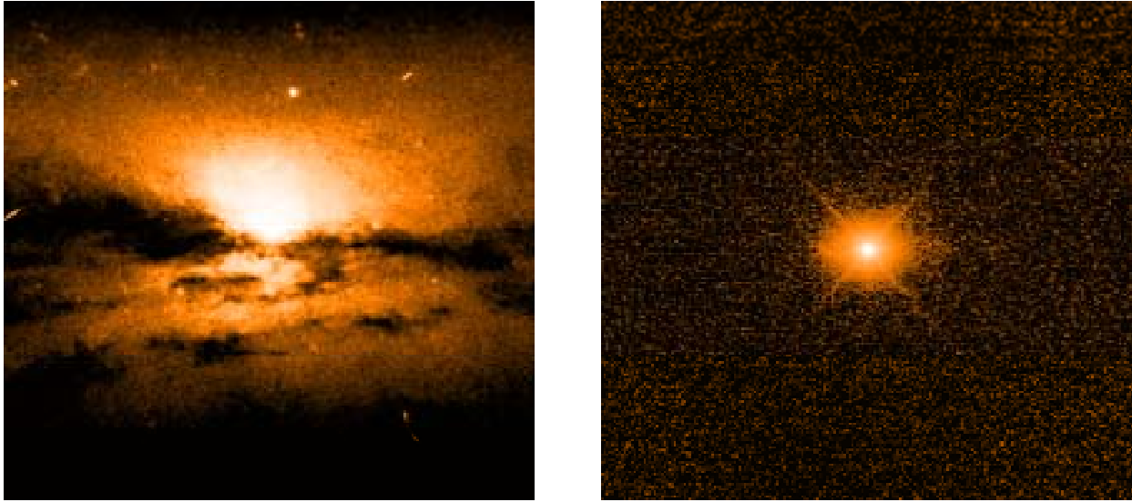
Fig. 3. NGC 5506 images of the central 35x45" by HST F606W (left) and NACO in Ks-band, 20x20" (right). Resolution of the NACO image is 57 mas. North is up, East, left.
