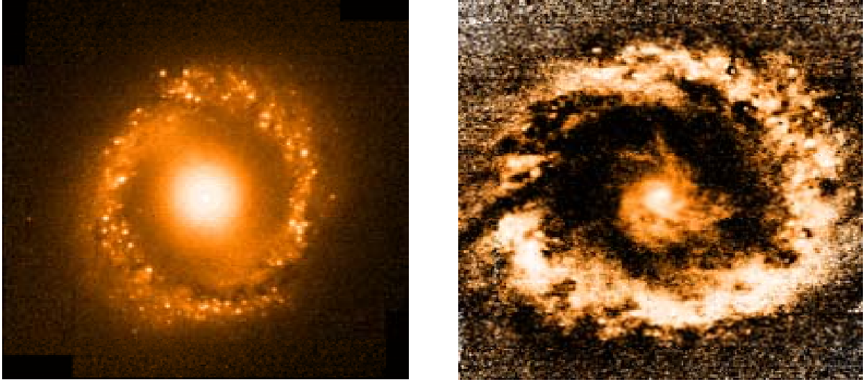
Fig. 2. Right: NGC1097 NACO Ks-band of the central 27x27 arcsec region; Right: NACO J-K image disclosing within the central 300 pc radius a fine spiral network of dust and gas spiraling toward the center. North is up, East to the left in both figures.
