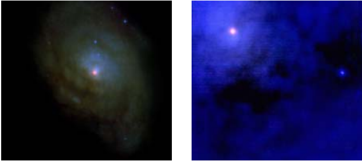
Fig. 1. Left: True colour image of Circinus, FoV = 27'' \times 27'' , combining HST F814W (blue) and NACO J- (green) and Ks-bands (red). Some of the stars used for astrometry and spatial resolution estimate are visible. Right: NACO J+H+K image of Centaurus A, FoV= 7'' \times 14'' . The star on the right side was used for astrometry and spatial resolution estimate. North up, East left in both figures.
