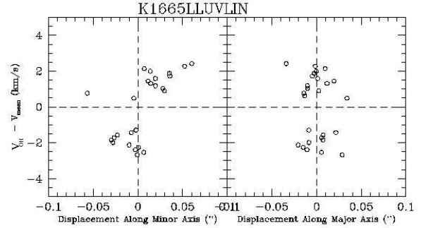
Fig. 2. OH 1665 MHz maser velocity plotted against the displacement along the minor axis of the outflow at a position angle of -45^\circ (left) and along the major axis at a position angle of 45^\circ (right).
