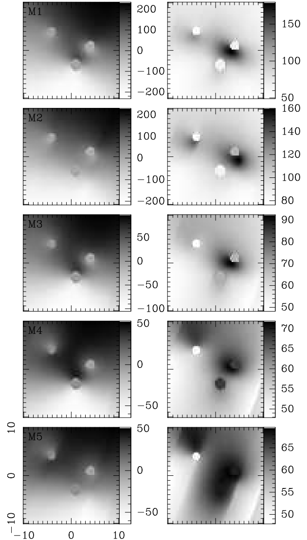
Fig. 11. Barycenter (left) and velocity dispersion (right) maps predicted from the five models described in the text (also see Tables 2 and 3). The two axes are labeled in arcseconds as offsets from a position in the middle of HH 2. The maps are shown with linear greyscales given in \text{km s}^{-1} by the bars to the right of each plot.
