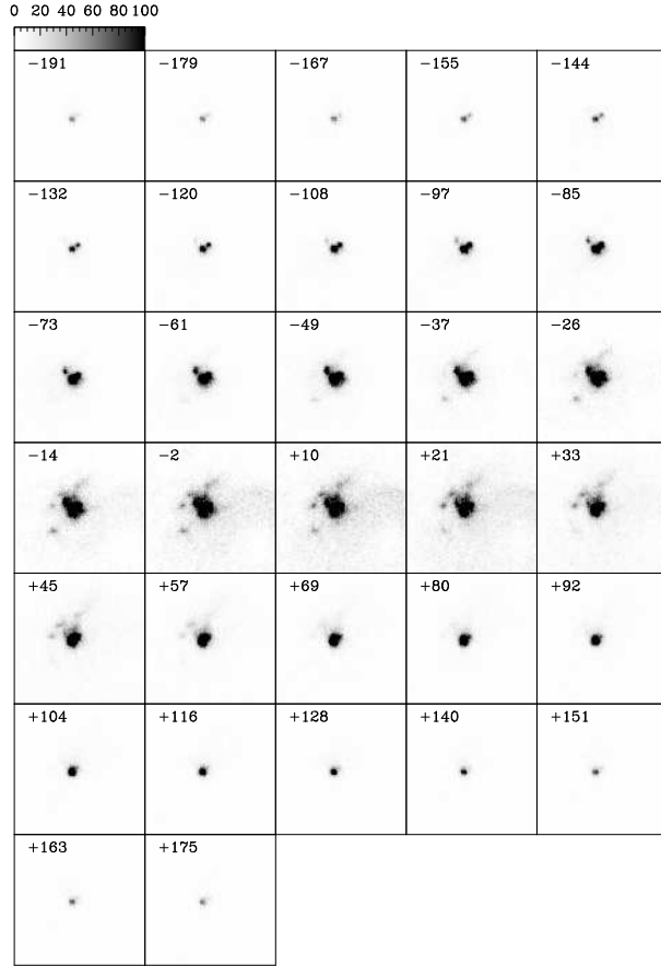
Fig. 5. H\alpha velocity channel maps corresponding to various radial velocities obtained from the Fabry-Perot data of HH 2. Labels correspond to the central heliocentric radial velocity of each channel (in \text{km s}^{-1} ).
