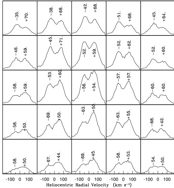
Fig. 10. H\alpha emission line profiles of HH 2H. The emission line profiles of each pixel (corresponding to 0.91'' \times 0.91'' ) are plotted as relative intensity (in counts) vs. heliocentric radial velocity. The spatial field presented in this figure is of 4.55'' \times 4.55'' and corresponds to the region of knot HH 2H. The observed emission line profiles were fitted with two Gaussian components. The central velocities of these Gaussian profiles are also indicated (in \text{km s}^{-1} ). North is up and East to the left.
