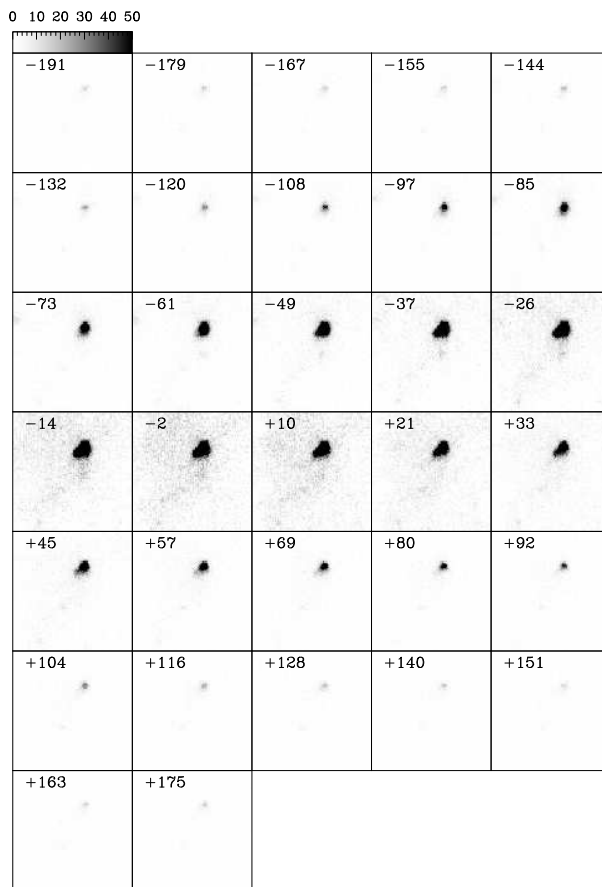
Fig. 3. H\alpha velocity channel maps corresponding to various radial velocities obtained from the Fabry-Perot data of HH 1. Labels correspond to the central heliocentric radial velocity of each channel (in \text{km s}^{-1} ). The maps are shown with a linear greyscale given by the bar (in counts).
