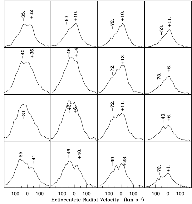
Fig. 9. \text{H}\alpha emission line profiles of HH 2A. The emission line profiles of each pixel (corresponding to 0.91'' \times 0.91'' ) are plotted as relative intensity (in counts) vs. heliocentric radial velocity. The spatial field presented in this figure is 3.64'' \times 3.64'' and corresponds to the region of knot HH 2A. The observed emission line profiles were fitted with two Gaussian components. The central velocities of these Gaussian profiles are also indicated (in \text{km s}^{-1} ). North is up and East to the left.
