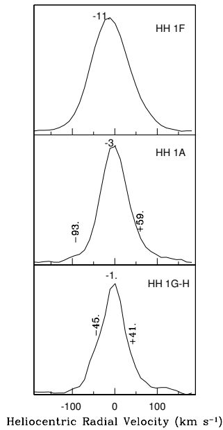
Fig. 7. Emission line profiles of HH1 F (top), A (center) G-H (bottom) obtained by integrating the emission over the knots. The relative intensities (in counts) as a function of the heliocentric radial velocities (in \text{km s}^{-1} ) are presented. The heliocentric radial velocities of the Gaussian components are also indicated (see the text).
