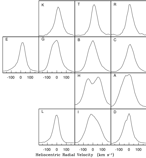
Fig. 8. Emission line profiles of several knots of HH 2 obtained by integrating the emission over the knots. The relative intensities (in counts) as a function of the heliocentric radial velocities (in \text{km s}^{-1} ) are presented.
