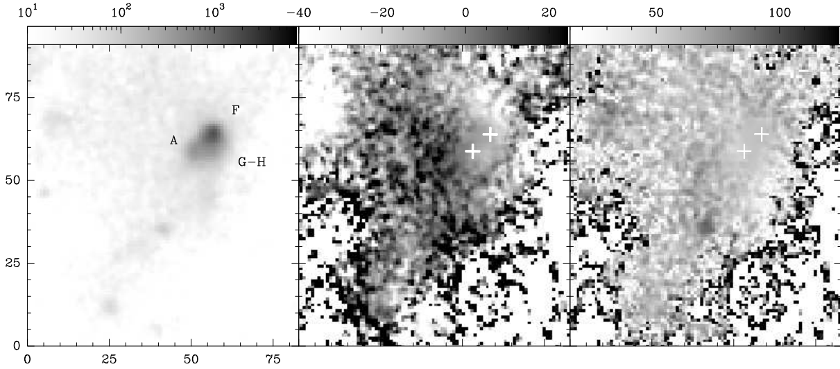
Fig. 4. Left panel: H\alpha map of HH 1. The observed knots are identified following the nomenclature of Herbig & Jones (1981) and Eisloffel et al. (1994). The greyscale of the maps is given by the bar (in counts). Central panel: H\alpha barycenter radial velocity map obtained from the position-velocity cube. The greyscale (linear, in \text{km s}^{-1} ) is given by the bar. Right panel: H\alpha line dispersion map obtained from the position-velocity cube. The greyscale (linear, in \text{km s}^{-1} ) is given by the bar. The crosses indicate the positions of condensations F and A. The two axes are labeled in arcseconds.
