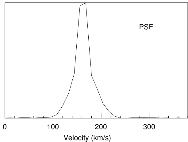
Fig. 1. The instrumental PSF obtained from the Neon line.
