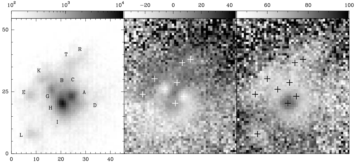
Fig. 6. As Fig. 4 but for HH 2. The crosses indicate the position of the knots of HH 2, with the exception of knots B, D, and I, which were not spatially resolved.
