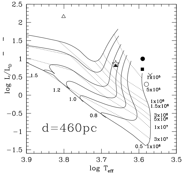
Fig. 4. Loci of the program stars in the HR diagram (HBC 498 filled triangle, DL Ori/G2 filled square, HBC 495 empty star, HBC 496 “X”, HBC 497 filled circle, IRS 5 empty circle and DL Ori/D empty triangle). Excluding IRS 5 (see text for details about this star), typical errors in temperature and luminosity are \varepsilon_{\log T} = 0.029 and \varepsilon_{\log L} = 0.075 , respectively.
