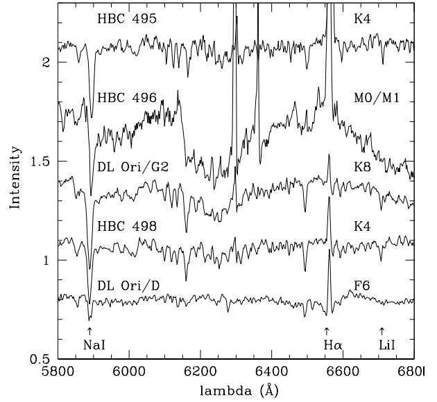
Fig. 2. Normalized spectra of the program stars, shifted arbitrarily along the intensity axis for convenience.
