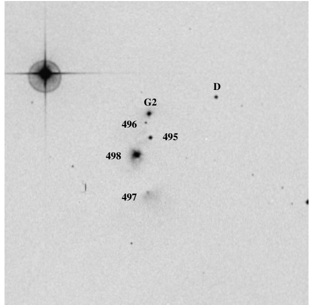
Fig. 1. POSS-red 10' \times 10' image of the HBC 498 region. North to the top and east to the left. The bright object at the left corner is the A0/A1 V star HD 37846.
