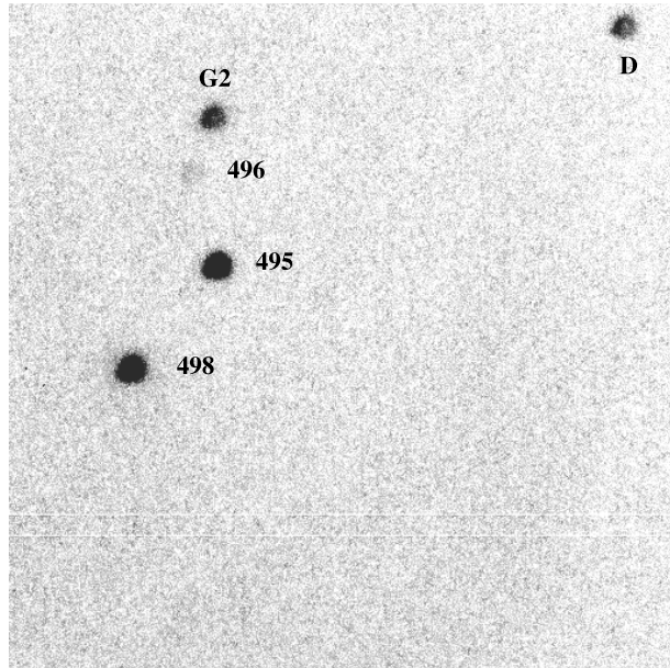
Fig. 3. Composite H\alpha image of the region of HBC 498 with an effective exposure time of 3600 s. Same orientation as Fig. 1. See text for details.
