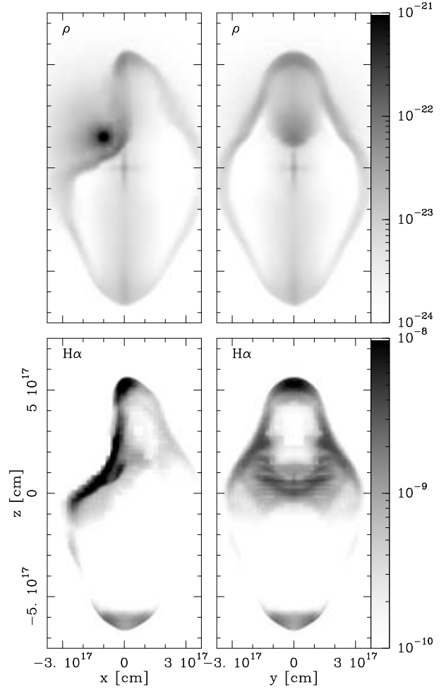
Fig. 2. Results obtained from model M1 for t_f = 1100 yr (see the text and table 1). The top frames show the density stratifications on the xz - (left) and yz -plane (right) with a logarithmic greyscale (given in g cm ^{-3} by the bar on the right). The bottom frames show the H \alpha maps obtained by integrating the H \alpha emission coefficient along the y - (left) and x -axis (right) with a logarithmic greyscale (given in erg cm ^{-2} s ^{-1} sterad ^{-1} by the bar on the right).
