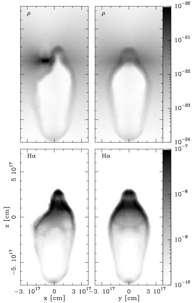
Fig. 4. Results obtained from model M3 for t_f = 1500 yr (see the text and Table 1). A description of the four frames is given in the caption of Fig. 1.
