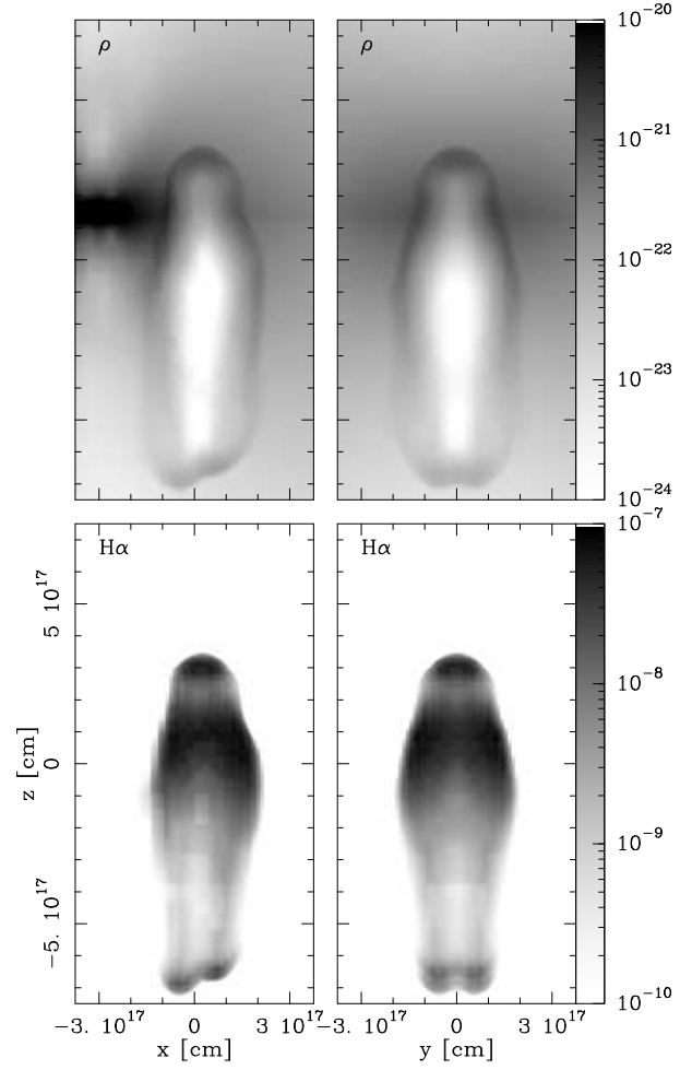
Fig. 6. Results obtained from model M5 for t_f = 2700 yr (see the text and Table 1). A description of the four frames is given in the caption of Fig. 1.
