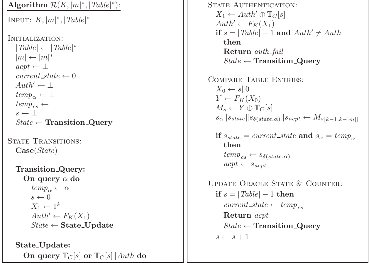
Figure 3: Oracle \mathcal{R} .
