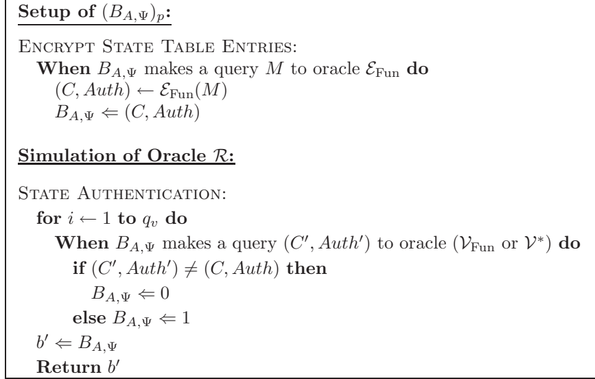
Figure 5: Adversary (B_{A,\Psi})_p
