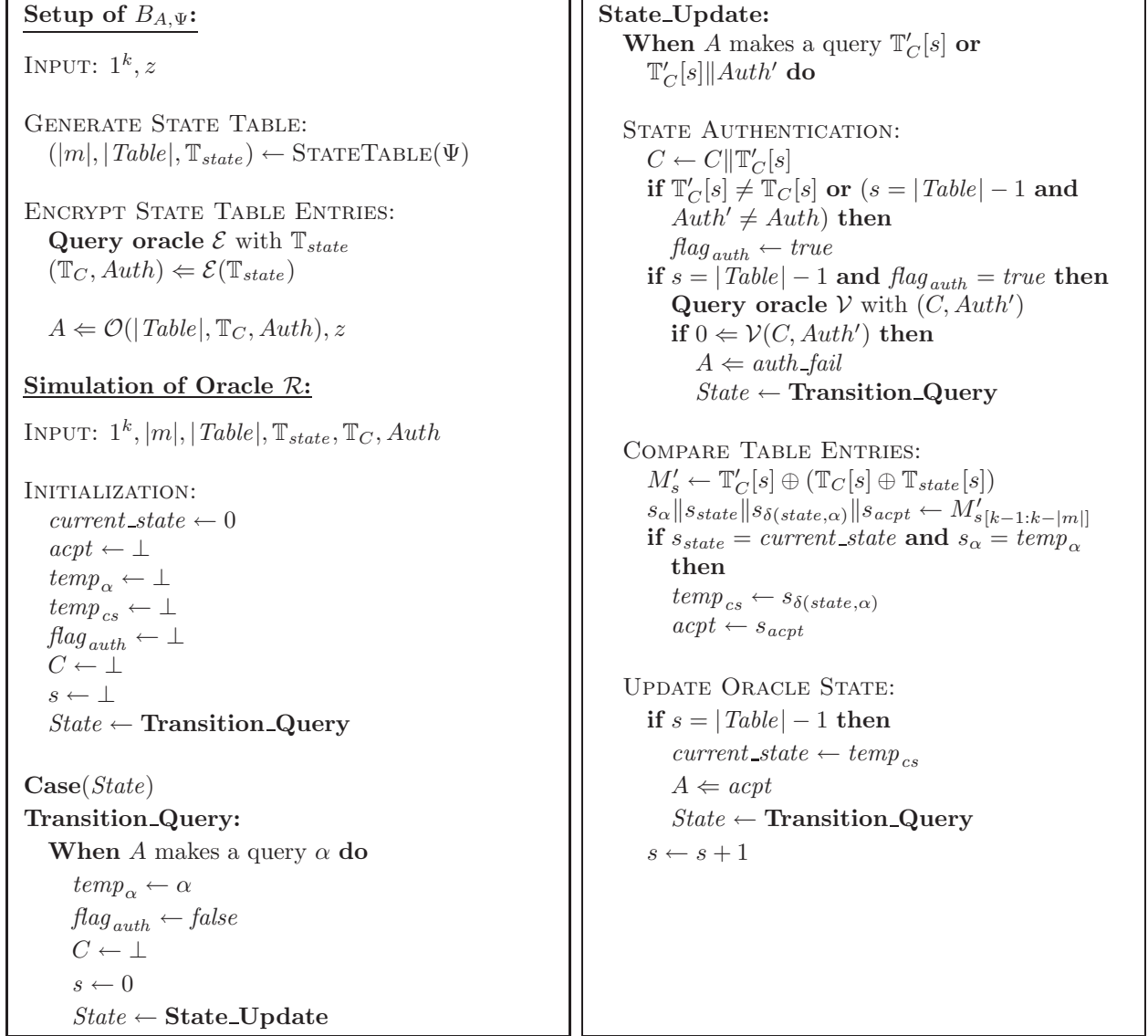
Figure 4: Adversary B_{A,\Psi} .
