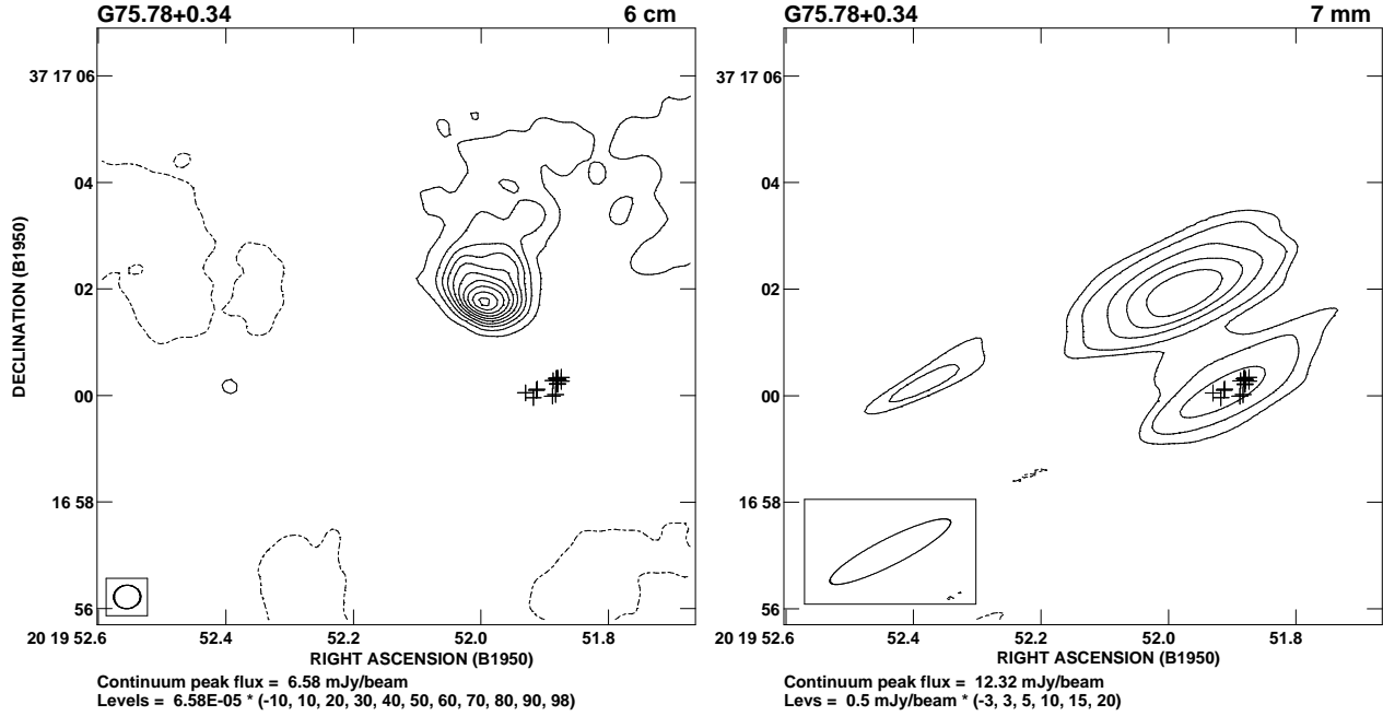
Fig. 3. Two views of the H II region G75.78+0.34. ( Left ) The original view, a 6 cm continuum snapshot made with the VLA (Wood & Churchwell 1989). The crosses indicate water maser positions, detected by Hofner & Churchwell (1996). No centimeter continuum emission was seen coincident with the maser clump. ( Right ) The same field, observed at 7 mm using the VLA (Carral et al. 1997). Millimeter wave continuum emission coincident with the maser clump is clearly present.
