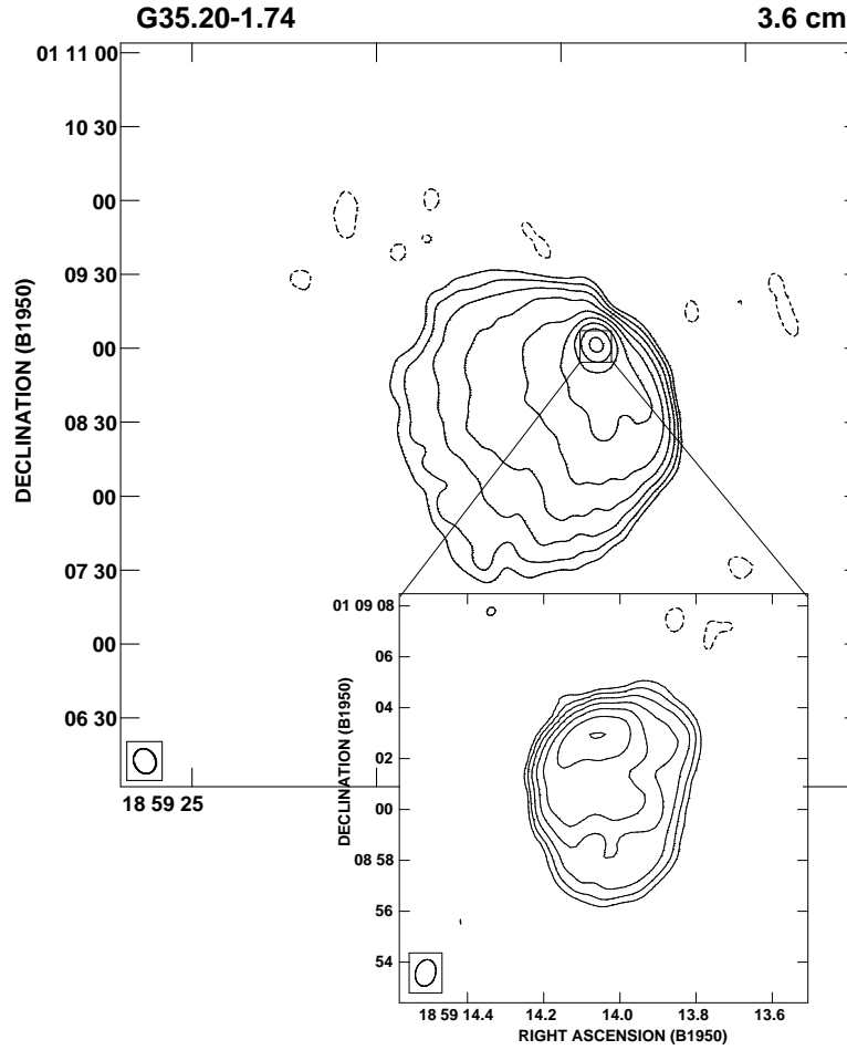
Fig. 2. Two views of the H II region G35.20–1.74. The original view (inset), made with sub-arcsecond resolution, was sensitive only to structures smaller than about 20'' (Wood & Churchwell 1989; Kurtz et al. 1994). Subsequent lower resolution observations, sensitive to structures up to 3' in size, show the full extent of the ionized gas in the region. The region has a cometary morphology at both arcsecond and arcminute scales.
