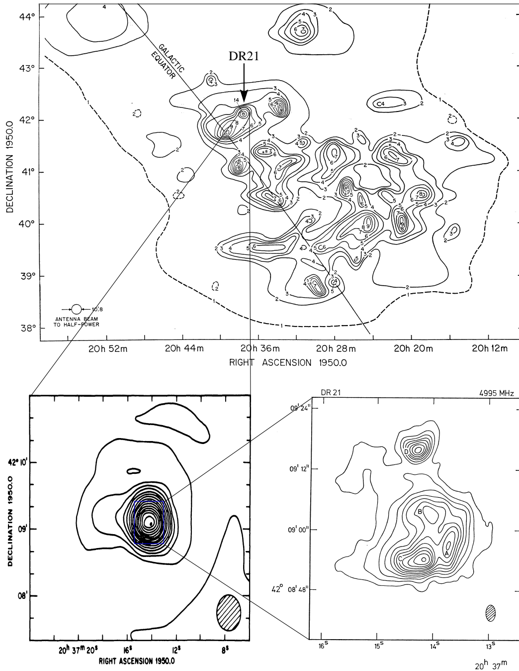
Fig. 1. This sequence of radio images shows the evolving view of (ultra)compact H II regions. Top , is the single-dish (10'8 beam) 5-GHz image of the Cygnus-X region, made by Downes & Rinehart (1966). The source DR21, indicated by the arrow, was unresolved and was the brightest source detected. Bottom left , is the DR21 region, imaged at 1.4 GHz with the Cambridge 1 Mile Array. The source is still unresolved, now with a beam of 34'' × 23''. Limits on the size and density lead this region to be classified as "compact." From Ryle & Downes (1967). Bottom right , is the same field, imaged with the Cambridge 5 km Array. The resolution is 3'' × 2''. At this level, structure within the "compact" H II region begins to emerge. The components A–D are now known as "ultracompact" H II regions. From Harris (1973).
