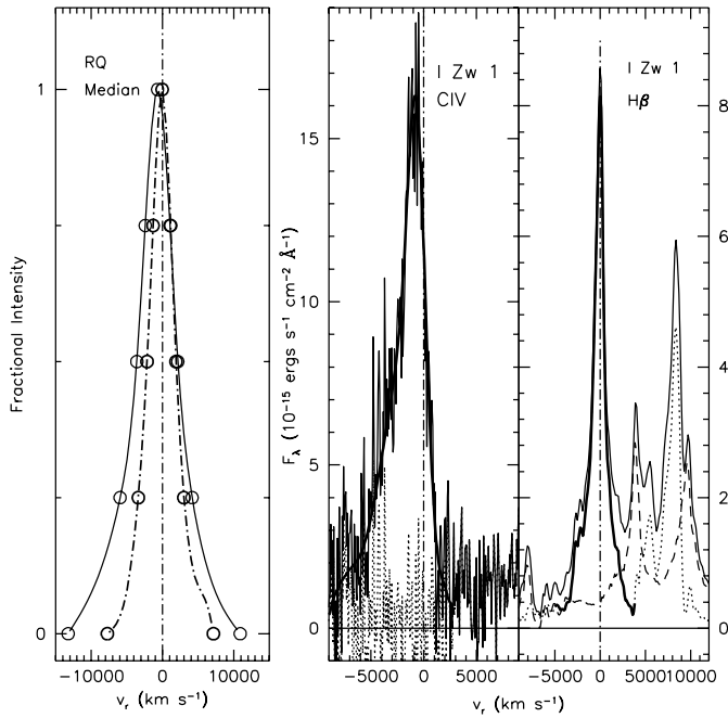
Fig. 1. Profiles of C IV \lambda 1549_{\text{BC}} (solid lines) and \text{H}\beta_{\text{BC}} normalized to the same peak intensity and constructed from median values of the radial velocities measured on the blue and red sides of the profiles for the 21 RQ AGN of Marziani et al. (1996) ( left panel ). Emission line profiles of C IV \lambda 1549 (middle panel) and \text{H}\beta ( right panel ) of the prototype NLSy1 galaxy I Zw 1, adapted from Marziani et al. (1996). The thick and the dotted lines trace \text{H}\beta and [\text{O III}]\lambda\lambda 4959,5007 after \text{Fe II}_{\text{opt}} (dashed line) subtraction.
