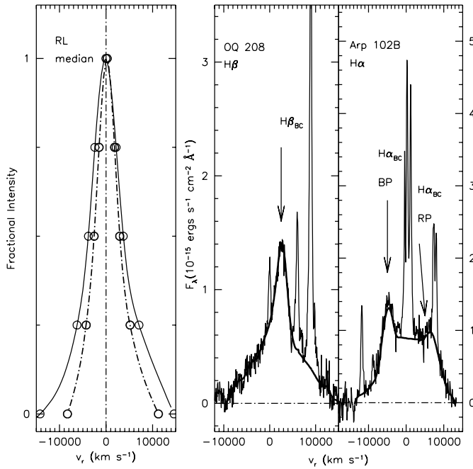
Fig. 2. Left panel: Profiles of C IV \lambda 1549_{BC} (solid lines) and H\beta_{BC} normalized to the same peak intensity and constructed from median values of the radial velocities measured on the blue and red sides of the profiles for the 31 RL AGN of Marziani et al. (1996). Middle panel: H\beta spectrum of OQ 208, showing a single, widely displaced H\beta_{BC} peak (adapted from Marziani et al. 1993). Right panel: H\alpha profile of the prototype of “wide-separation double peakers” Arp 102B. Unpublished spectrum obtained at the 1.82-m telescope of the Asiago observatory on March 25, 1989. The thick solid line traces H\beta_{BC} .
