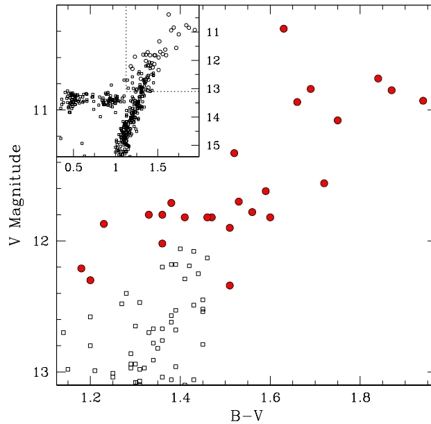
Fig. 1. A color–magnitude diagram of M4, with photometry from Cudworth & Rees (1990) showing the positions of our program stars in solid circles. The inset diagram shows the program stars with respect to all of the Cudworth & Rees (1990) M4 stars of magnitude \leq 15.5 .
