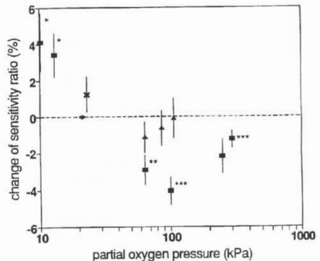
FIG. 3—Influence of PO 2 in the inspired gas under normobaric and hyperbaric conditions. Bars are 2 × SE. ■ Normobaric abnormal FI O 2 (PO 2 = 10 kPa with 5 subjects (Ss) and 11 sessions in total; PO 2 = 13 kPa, 5 Ss, 8 sessions; PO 2 = 65 kPa, 5 Ss, 9 sessions; PO 2 = 100 kPa, 7 Ss, 9 sessions), and HBO 2 (250 kPa, 2 Ss, 2 sessions; 300 kPa, 6 Ss, 10 sessions). ▲ Hyperbarism with FI O 2 = 0.21 (all pressures 4 Ss, 7, 8, and 5 sessions from low to high pressure). × Enriched, hyperbaric N 2 mixture (4 Ss, 8 sessions) + control value. * P < 0.05 , ** P < 0.01 , and *** P < 0.001 (one-tailed t test). The data obtained with 10 and 13 kPa taken together yield a very significant increase of rgSR ( P < 0.001 , one-tailed t test).
