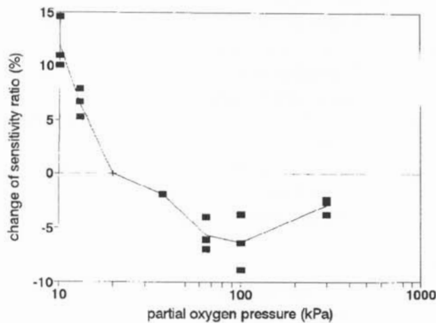
FIG. 2—Influence of oxygen on rgSR expressed in percent (vertical axis) as function of PO 2 (horizontal axis) under normobaric (10–100 kPa) and hyperbaric conditions (HBO 2 at 300 kPa). Each square denotes one session, depicting rgSR exp - rgSR con (see Methods). The subject, same as in Fig. 1, showed the largest effects to a change of PO 2 . Since the temperature in the hyperbaric chambers varied about 4°C during a session, the rgSRs obtained under pressure were corrected for the temperature coefficient of the Oscar (0.07 OU/°C) + control value.
