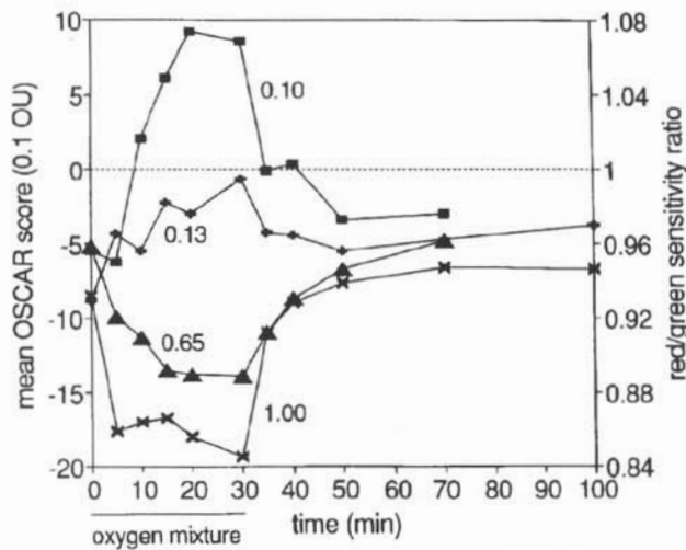
FIG. 1—Influence of normobaric O 2 -N 2 mixtures on rgSR expressed in Oscar units (vertical axis) as a function of exposure time. (One subject, each curve mean of three sessions.) O 2 -N 2 mixtures with a FI O 2 of 0.13 and 0.10 are equivalent to altitudes of 3,900 and 5,900 m, respectively. Figures marking the curves denote FI O 2 .
