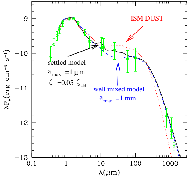
Fig. 3. SED of disk models with standard values of \dot{M} , \alpha , central star properties and different assumptions for the dust: well mixed ISM dust (dotted line), well mixed grains with a_{max} = 1 mm (dashed line) and dust settling, with an atmospheric value of a_{max} = 1 \mu\text{m} and a mid-plane value of 1 mm (solid line). The points represent the median observed SED of CTTS in Taurus (D'Alessio et al. 1999).
