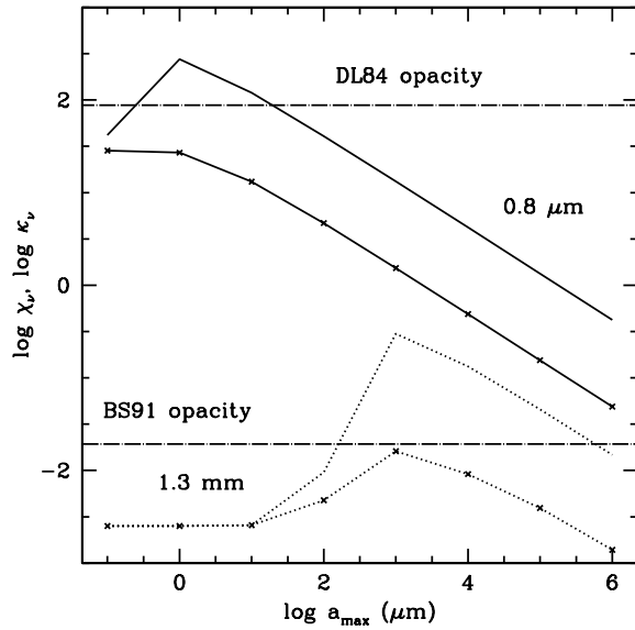
Fig. 1. Dust opacity at \lambda = 0.8 \mu\text{m} (solid lines) and 1.3 mm (dotted lines), for a distribution of sizes n \sim a^{-3.5} , with a_{\text{min}} = 0.005 \mu\text{m} and different a_{\text{max}} . The curves with dots correspond to the true absorption coefficient only, \kappa_\nu , and the curves without dots include the scattering coefficient, \chi_\nu = \kappa_\nu + \sigma_\nu . The horizontal lines represent the opacity for ISM dust at 0.8 \mu\text{m} (labelled DL84 after Draine & Lee 1984) and the opacity proposed by BS91 at 1.3 mm (labelled BS91)
