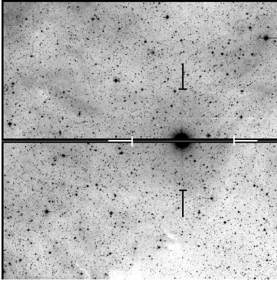
Fig. 2. H\alpha + [NII] deep image of the region around the PN NGC 7027. The WFC cover a total field of 34' \times 34' but we present here only the image in the CCD's number 4 and 1, between which the PN was located. The lines mark the circular region detected (not well seen in this b/w image). North at the top.
