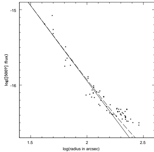
Fig. 1. Observed [OIII] flux (see text) as a function of the distance to NGC 7027. The continuous line represent the extrapolation until 300'' of the King profile and the dashed line, the sum of the King profile and the diffuse galactic background.
