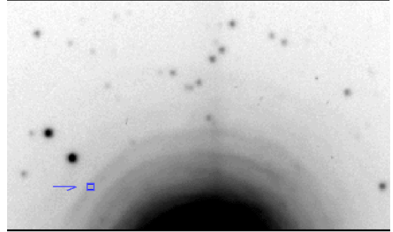
Fig. 3. [OIII] image of the rings around NGC 7027. The rings are observed in both images, but in [OIII] the contrast is better. The marked ring is at 36'' from the center of the PN (at 11'' below the limit of the image).
