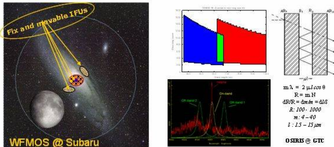
Fig. 7. WFT aims for complementary field and spectral coverage. Full wavelength range coverage, with carefully chosen spatial sampling, can be achieved by combining the sparse, point-like apertures of WFMOS (a project for the Subaru telescope) with a deployable and central IFU (left). On the other hand, full spatial coverage scanning a finite wavelength range is possible with narrow-band tunable imagers like OSIRIS on GTC (right panel).
