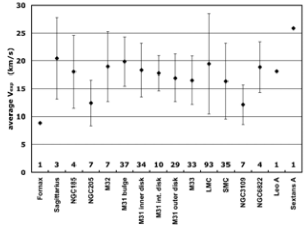
Fig. 1. For each galaxy, the point indicates the mean expansion velocity measured for its PN population; the error bars indicate the standard deviation of the expansion velocity distribution, and the numbers along the bottom axis indicate the number of PNe observed. We adopt the half-width at half-maximum as our measure of expansion velocity. Although this measure is arbitrary, most of the PNe have Gaussian line profiles at the S/N we achieve. The data for the Magellanic Clouds were taken from the literature (Dopita et al. 1985; Dopita et al. 1988), but analyzed in the same manner as the other data.
