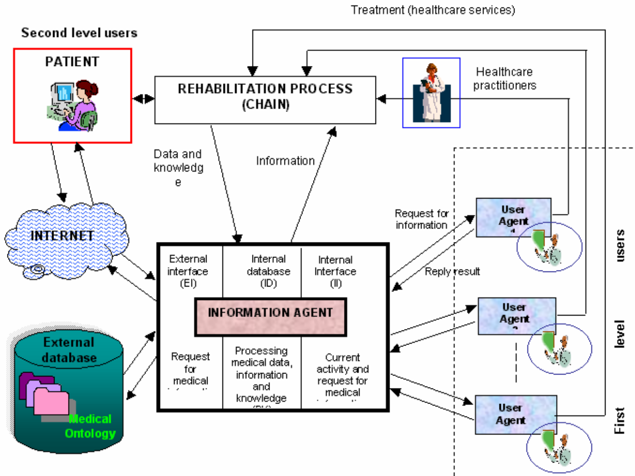
Figure 2: The architecture of the information agent-based model for a rehabilitation VN
