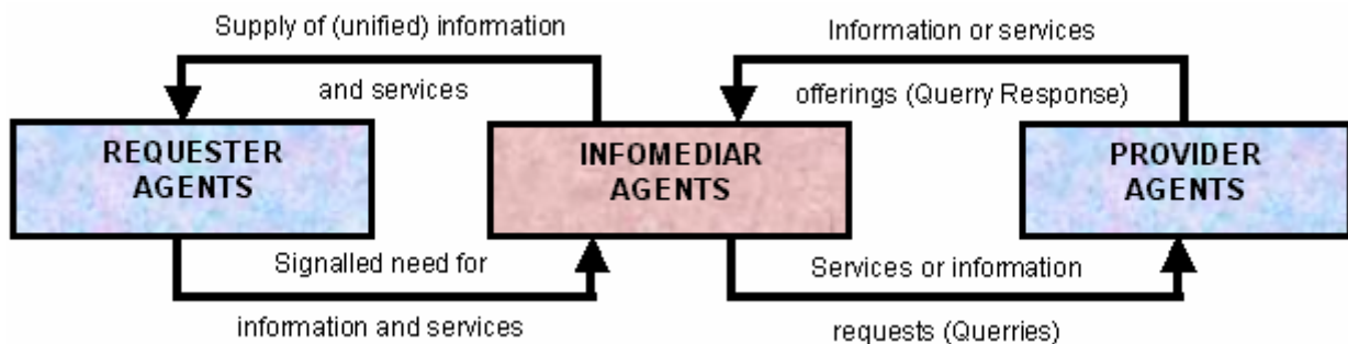
Figure 1: Architecture of an agent-based model
