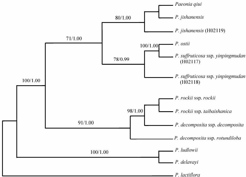
Fig. 1. The 50% majority-rule consensus tree of two MP trees based on Adh1A , Adh2 and GPAT (Tree length = 559, CI = 0.8927, RI = 0.7196). The numbers near branches are bootstrap percentages followed by Bayesian posterior probabilities.
