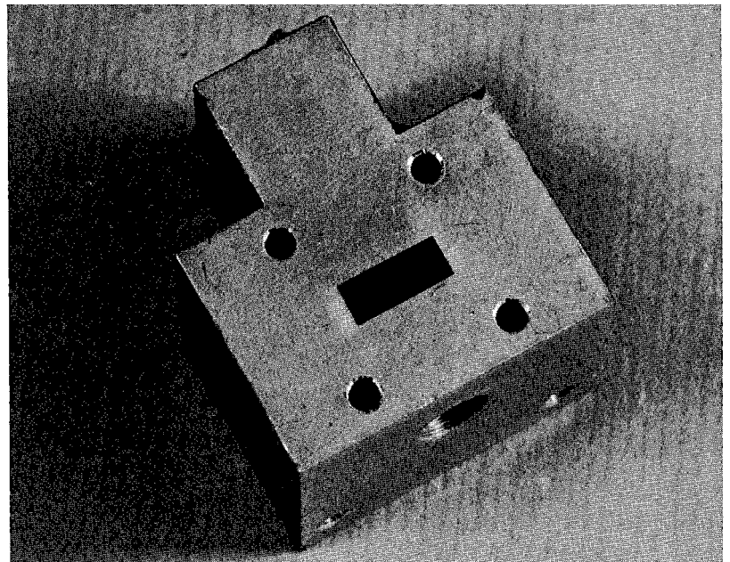
Figure 3: Waveguide in 6061 aluminium alloy1
