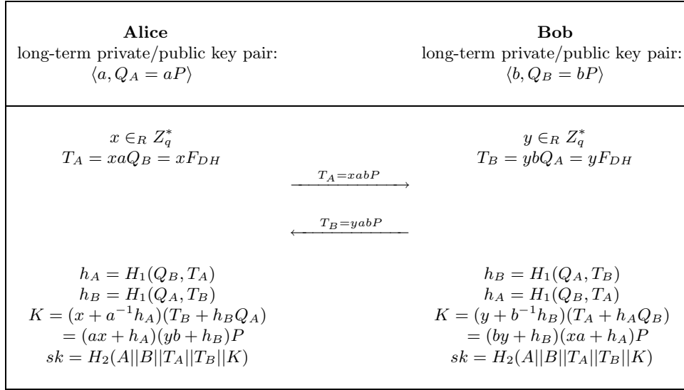
Fig. 19. The Enhanced MTI/C1 Protocol
