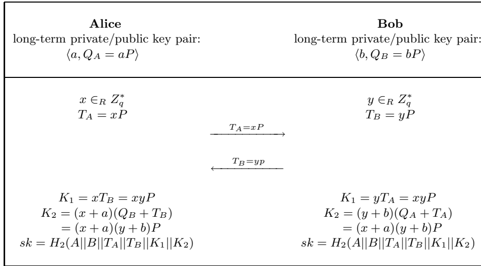
Fig. 18. nID-SYL: A New Authenticated Diffie-Hellman Protocol
