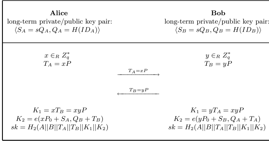
Fig. 17. The SYL Protocol [40]
