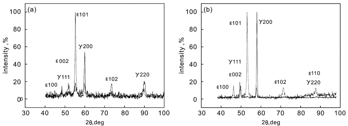
Fig. 5 XRD patterns of TIG remelted surface and ground surface before and after cavitation test (a) TIG remelted, (b) ground
