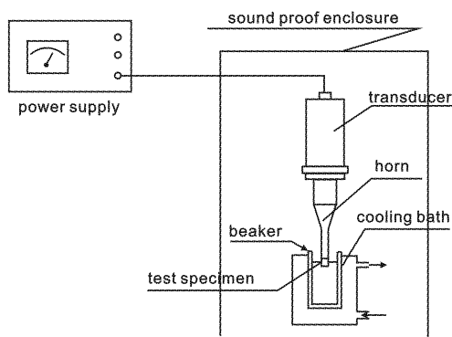
Fig. 1 Schematic diagram of cavitation vibratory test
