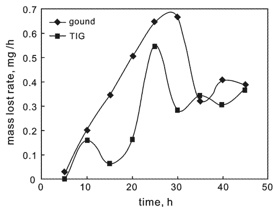
Fig. 3 Mass lost volume via cavitation erosion time
