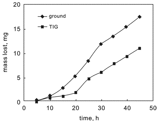
Fig. 2 Mass lost rate via cavitation erosion time
