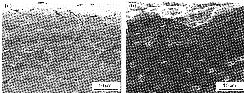
Fig. 6 Cross-sectional SEM images of specimen after cavitation-erosion test (a) TIG remelted, (b) ground
