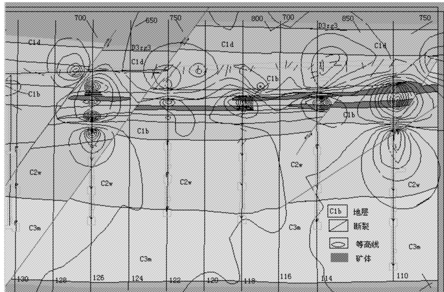
图3 会泽麒麟厂铅锌矿深部 1571 中段图异常预测与实际比较图 Fig.3 Comparing map of forecast and actual of 1571 middle segment in Huize Qiling Factory Pb-Zn mine deep part
