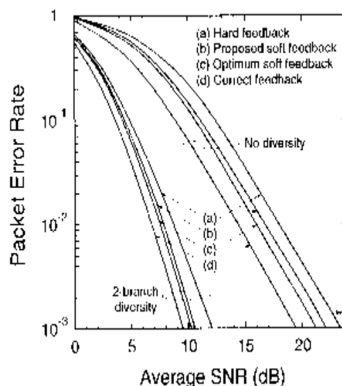
Fig. 2. PER performance of different DFE schemes.
