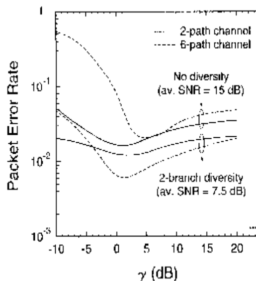
Fig. 3. Diversity influence on PER performances.
