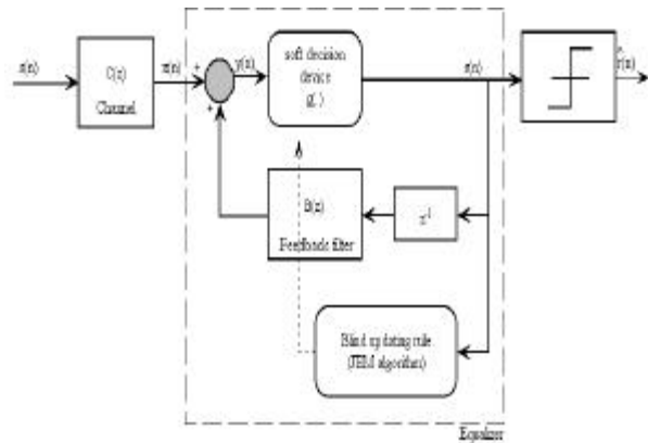
Fig. 1. Block scheme of the DFE structure.
