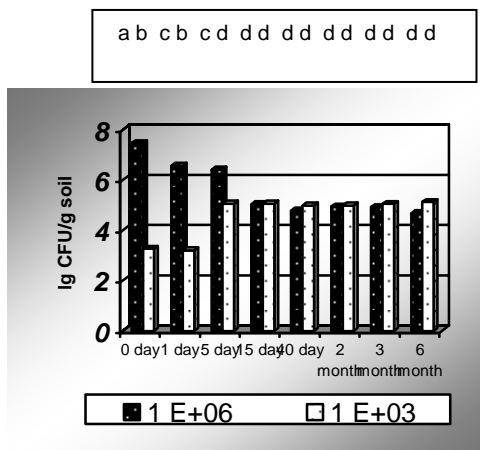
Fig. 2. Population dynamics of S. cirsi in sterile soil at initial concentrations of close to 1 E + 03 and 1 E + 06 conidia g -1 of soil (in 10 g of soil). Bars marked with the same letter are not significantly different.
