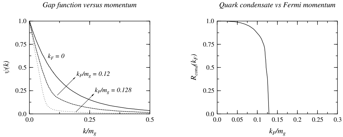
FIG. 1: Left panel: The gap function \psi(k) as a function of momentum for different values of Fermi momenta. Right panel: The ratio of the in-medium to vacuum quark condensates as a function of the Fermi momentum. All dimensional quantities are scaled by m_g .
