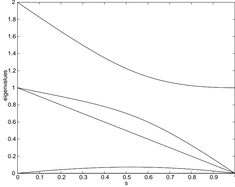
Figure 5: The four eigenvalues of \tilde{H}(s) associated with the 2-bit imply clause.
