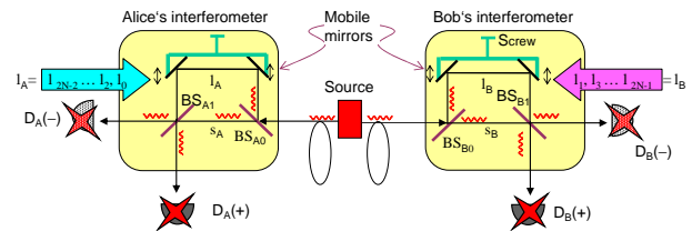
FIG. 2: Diagram of a 2-particle experiment using interferometers: The source emits photon pairs produced by down conversion. Photon A (frequency \omega_A ) enters Alice's interferometer to the left and gets detected after leaving the beam-splitter BS_{A1} , and photon B (frequency \omega_B ) enters Bob's interferometer to the right and gets detected after leaving the beam-splitter BS_{B1} . The detectors are denoted D_A(+) , D_A(-) , and D_B(+) , D_B(-) , and correspondingly we say that the detections give the values (a, b \in \{+1, -1\}) . Each interferometer consists in a long arm of length l_i , and a short one of length s_i , i \in \{A, B\} . Bell experiments use N different values of l_A ( l_0, l_2, \dots, l_{2N-2} ) and N values of l_B ( l_1, l_3, \dots, l_{2N-1} ), with N \geq 2 . \Phi is the phase parameter depending on settings l_A, l_B on both sides of the setup. In order to have entanglement exhibiting nonlocal correlations in Alice's and Bob's labs only the path pairs: (s_A, s_B) and (l_A, l_B) can constructively contribute to the correlated outcomes, where (s_A, s_B) denotes the path defined by the two short arms, and (l_A, l_B) that by the two long arms. This imposes conditions to the frequency bandwidths and path alignments.
