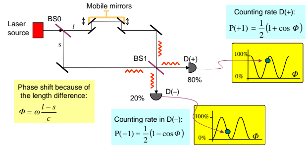
FIG. 1: Single particle interference: Laser light of frequency \omega emitted by the source enters an interferometer through beam-splitter (half-silvered mirror) BS0 and gets detected after leaving beam-splitter BS1. The light can reach each of the detectors D(+) and D(-) by the paths l and s ; the path-length l can be changed by the experimenter at will.
