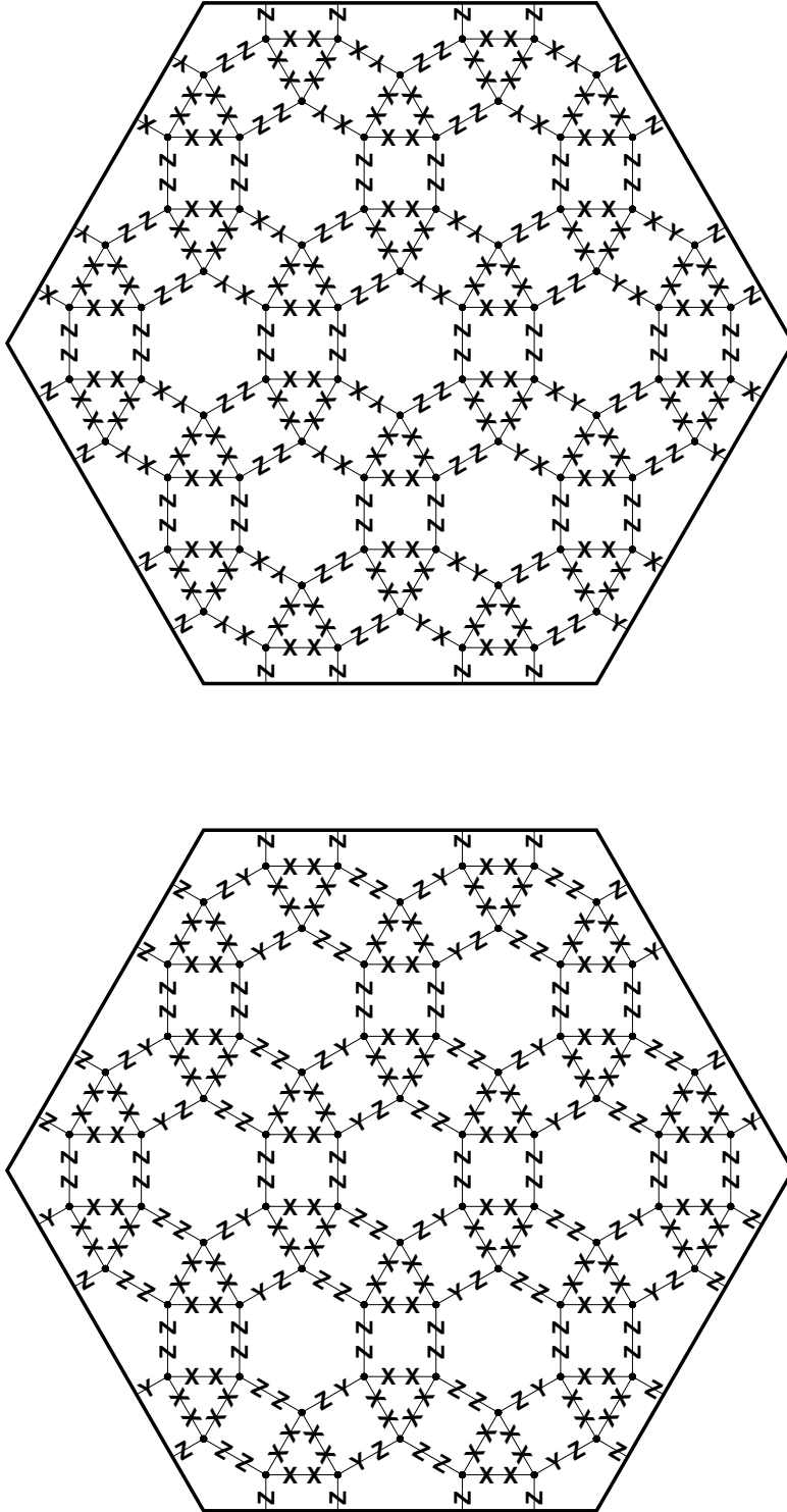
FIG. 15: A figure illustrating two labelings of the rhombihexadeltile tiling (on a radius 2 lattice) that result in a quantum code with distance 4 and sixteen when applied to a radius 3 lattice.
