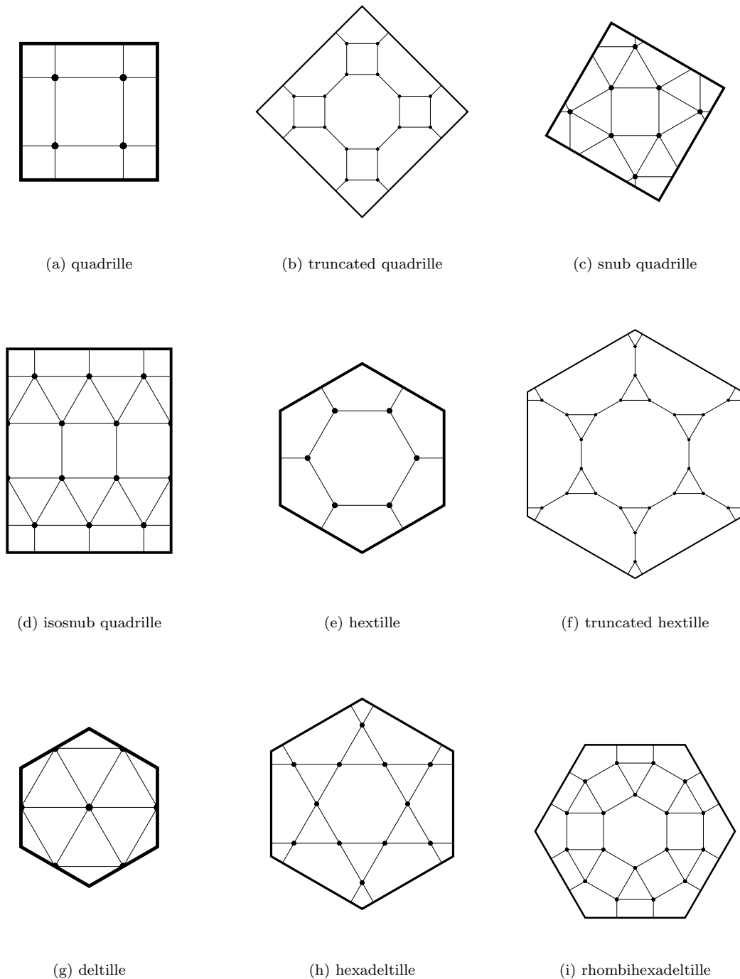
FIG. 2: A figure illustrating how we placed the centers and boundaries for each of the tilings that we scanned. The boundaries are periodic, so that edges that pass through one side of the boundary wrap around to the opposite side. Edges and vertices on a boundary are merged with the corresponding edges and vertices on the opposite edge. Note that under this scheme there can be no vertices on a corner. For most tilings this will never happen, but it turns out that in the case of the deltille tiling there are vertices on the corners when the radius (smallest distance from the center to the boundary) is three times the radius of the unit cell; we thus ignore deltille tilings of these sizes.
