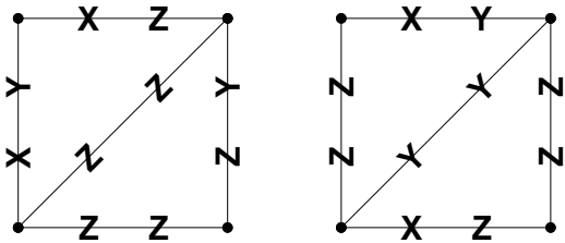
FIG. 1: A figure illustrating two possible labelings of a graph, which correspond to two possible choices of 2-body measurements. In both graphs we see that there are four vertices and five edges, which indicates that our system is constrained to have four qubits and five 2-body measurement operators. The edges (without the labels) indicate the pairs of qubits on which the 2-body measurement operators are constrained to act within our system. Within these constraints, we see in this figure two possible choices of measurement operators as specified by the two labelings of the edges of the graph.
