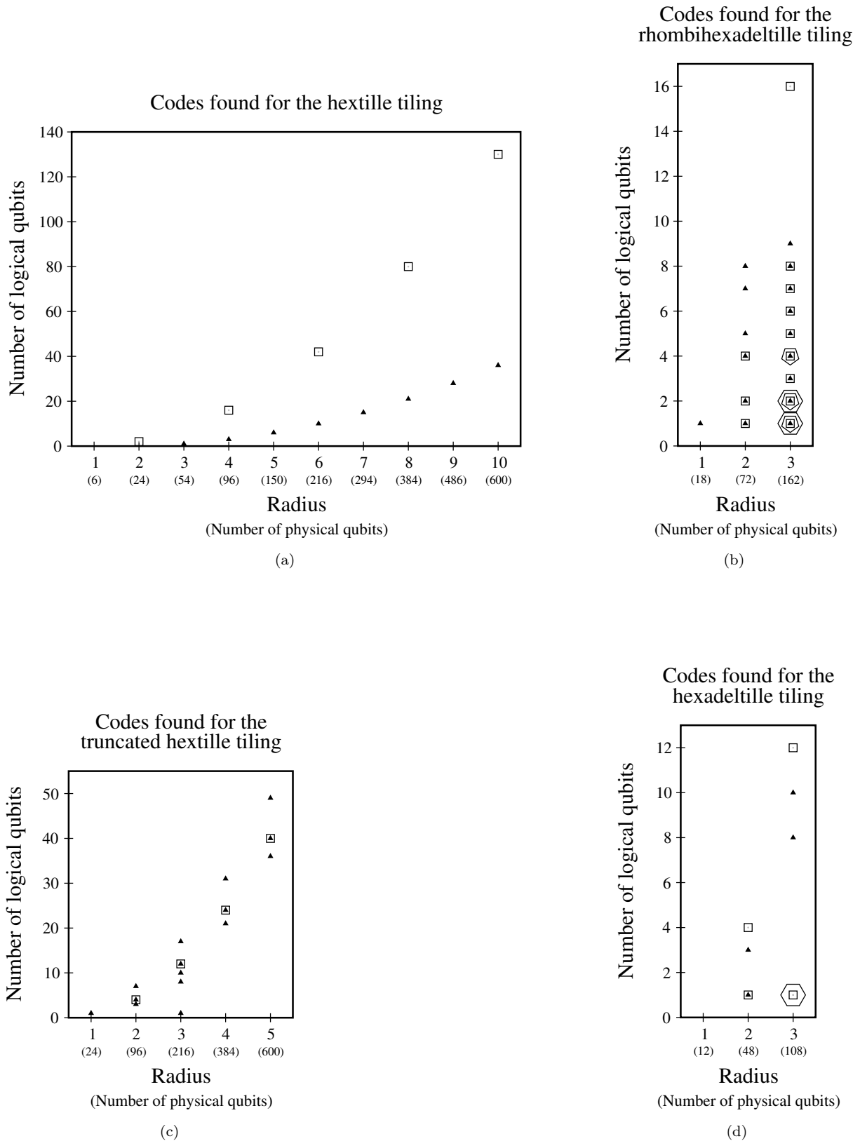
FIG. 4: A figure containing plots of the results from scanning the (a) hextille, (b) rhombihexadeltile, (c) truncated hextille and (d) hexadeltile tilings. See the caption of Figure 3 for an explanation of how to interpret these plots.
