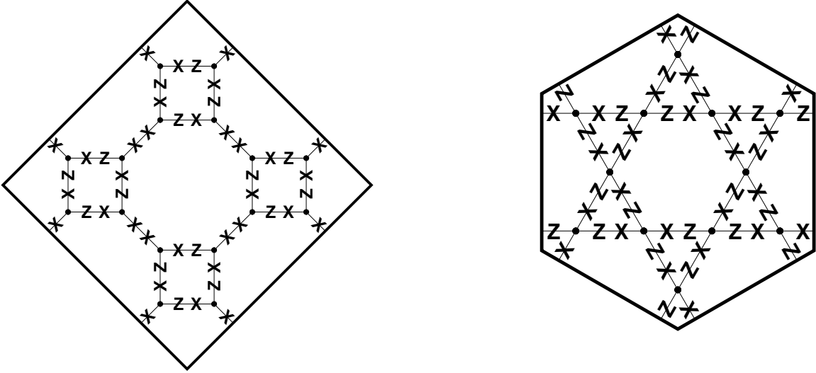
FIG. 13: A figure illustrating one of the labelings of the hexadeltile tiling (on a radius 1 lattice) that results in quantum code whose distance grows with the size of the tiling.
