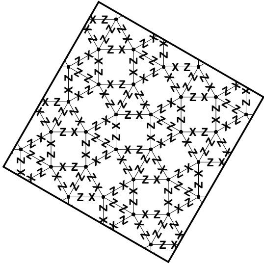
FIG. 7: A figure illustrating a labeling of the snub quadrille tiling (on a radius 2 lattice) that results with distance 4 and a number of distance logical qubits proportional to the square of the radius of the labeling.
