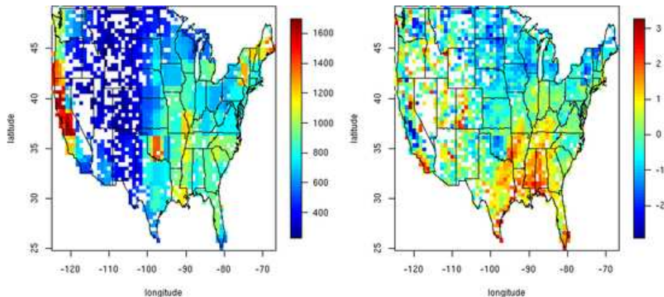
FIG. 4. Simple regression model including elevation: \text{Log}(\text{Point}) \sim \text{Grid} + \text{Elevation} using the NCEP grid cell data.
