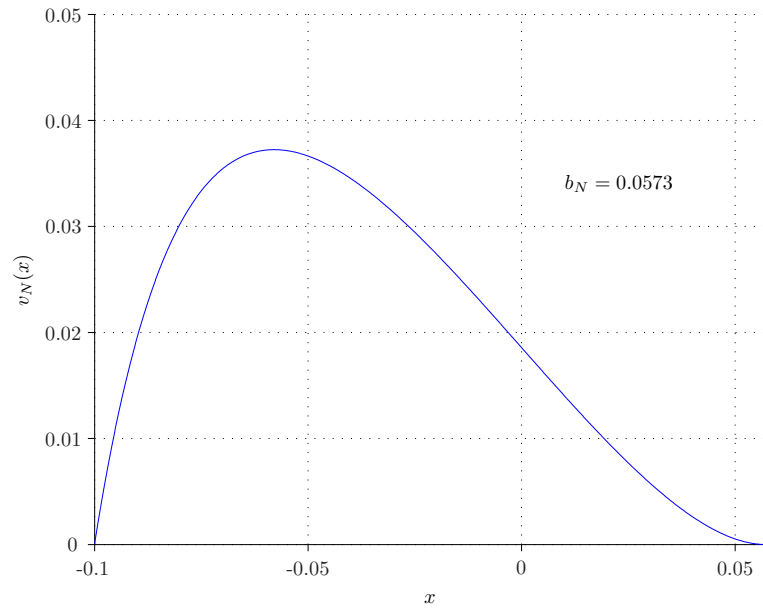
FIGURE 3.2. The solution (v_N, b_N) when a = -0.1 , \lambda = 10 , \sigma = 0.2 , \mu = \frac{\sigma^2}{0.005} , \gamma = 0.02 and J = 0.05 .
