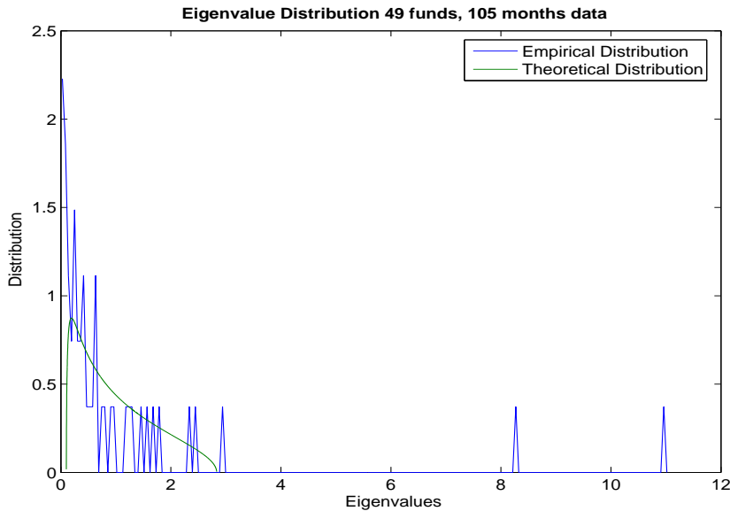
Fig. 1. Spectral Distribution for equally weighted Hedge Fund correlation matrix
