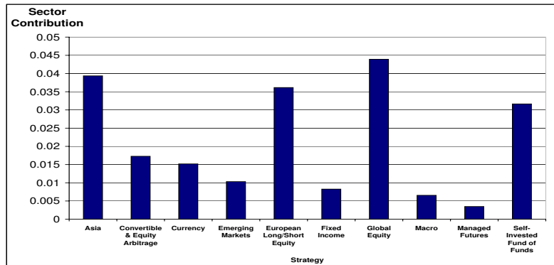
Fig. 8. Strategy Contribution, 2nd largest eigenvalue
