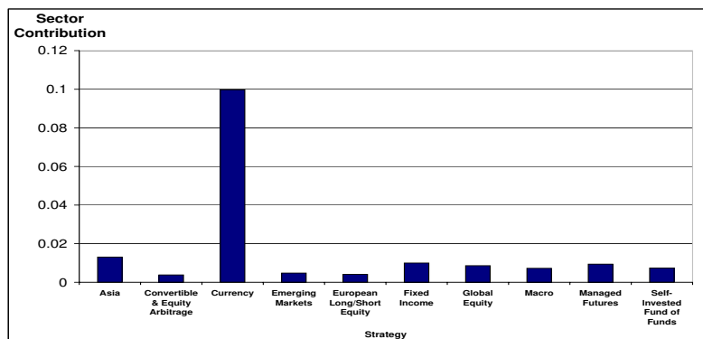
Fig. 9. Strategy Contribution, 3rd largest eigenvalue
