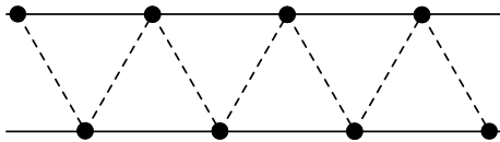
Figure 1: Configuration of the system in optical lattice implementation. Tunneling between the nearest three sites (black points) in a triangle gives rise to the triplet interaction term.
