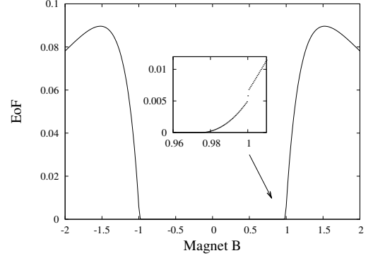
Figure 2: The EoF is shown as a function of the magnetic field strength B . The entanglement is born at B_E \simeq 0.9767 , and a sudden change happens at the critical point.
