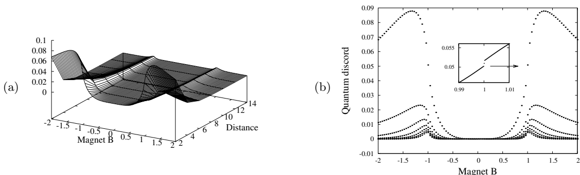
Figure 3: The quantum discord is plotted versus B and R where B is the magnetic field strength parameter and R is the site's number which correlates with site 0.
