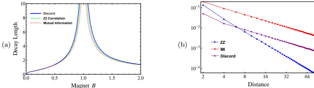
Figure 4: (Color online) (a) The decay length of quantum correlations (quantum discord, mutual information, and the correlation function \langle \sigma_0^z \sigma_R^z \rangle ) are plotted versus magnetic field strength B . (b) The decay behaviour at B = 1 . The correlations decay as \sim R^{-\xi} . We all take R as even.
