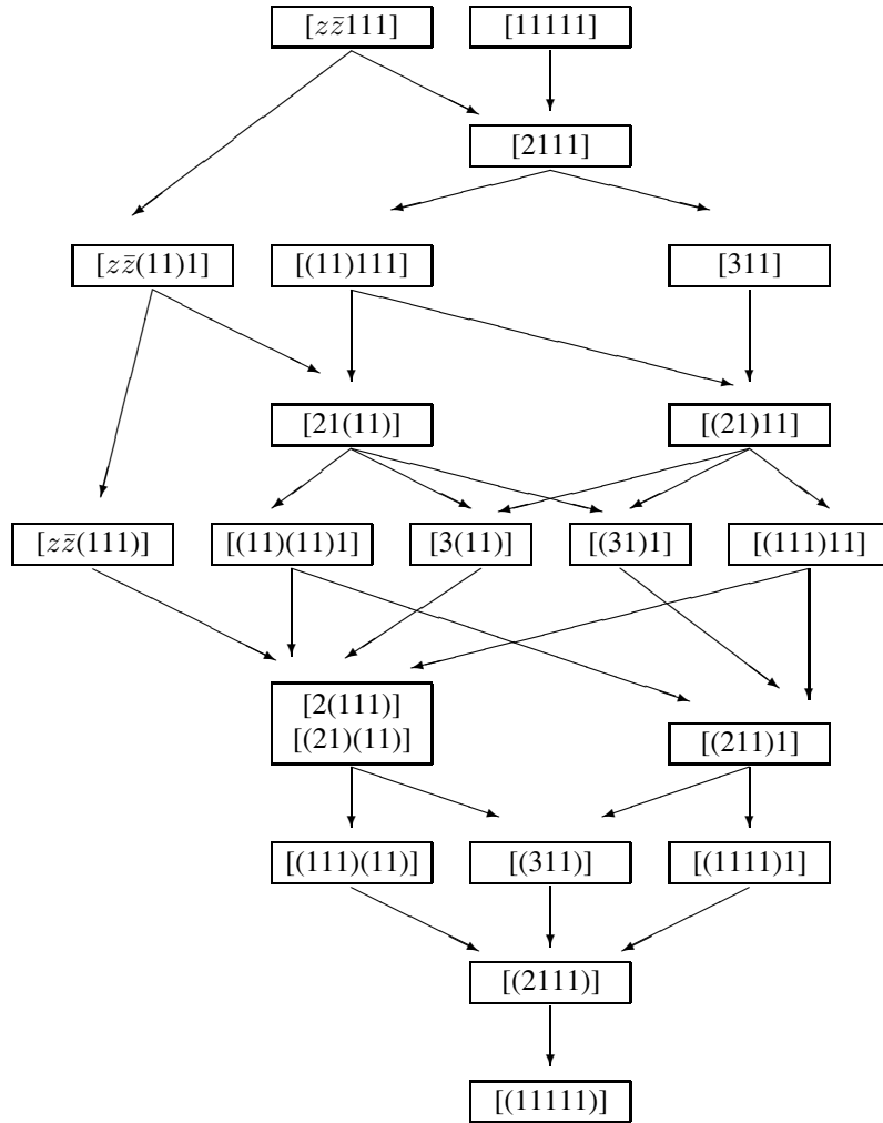
Figure 2. Diagram for the limits of the Segre types of R_b^\alpha in 5-D Lorentzian spaces.
