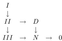
Figure 1. Limiting diagram for the Petrov types in 4–D.
