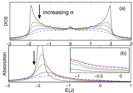
FIG. 1: DOS (a) and absorption spectra (b) for Lévy disorder with \alpha = 1/2 and disorder strengths \sigma = 0.01J, 0.1J, 0.2J, 0.5J , and J . The arrows mark the curves in order of increasing \sigma .
