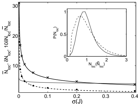
FIG. 3: The average, \bar{N}_{\text{loc}} , (crosses) and the standard deviation, \delta N_{\text{loc}} , (dots) of the localization length distribution P(N_{\text{loc}}) as functions of \sigma for Lévy disorder with \alpha = 1/2 . The thick solid and dashed lines are power-law fits, respectively (see text). The thin solid line gives 10(\delta N_{\text{loc}}/\bar{N}_{\text{loc}}) , while the inset shows the localization length distributions for \sigma = 0.001J (dashed) and for \sigma = 0.1J (solid).
