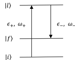
FIG. 1: Stimulated Raman scattering. |i\rangle , |l\rangle , and |f\rangle represent the initial state, the intermediate state, and the final state, respectively. A circular polarized photon with polarization \epsilon_+ and frequency \omega_+ is absorbed, and a circular polarized photon with polarization \epsilon_- and frequency \omega_- is emitted. All the states |i\rangle , |l\rangle , and |f\rangle are the entangled states of the N atom system.
