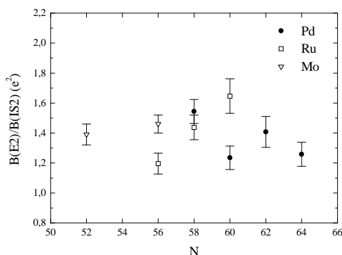
Figure 4. Ratios B(E2)/B(IS2)e^2 for ^{104,106,110}\text{Pd} , present work, in comparison with the ones obtained for ^{100,102,104}\text{Ru} [2] and ^{94,98}\text{Mo} [1].
