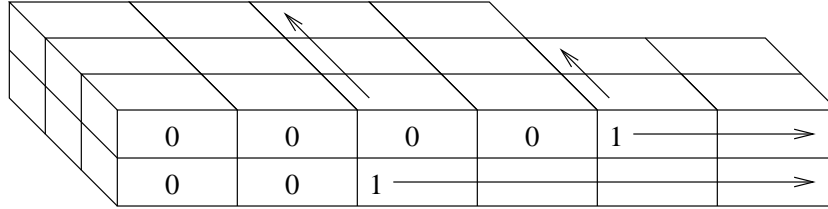
FIG. 6a. \mu = (3, 2) , Level 0
