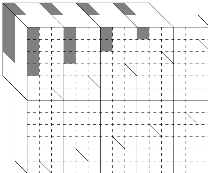
FIG. 3a. \mu = (2^{m_2}, 1^{m_1}) , Level 0
