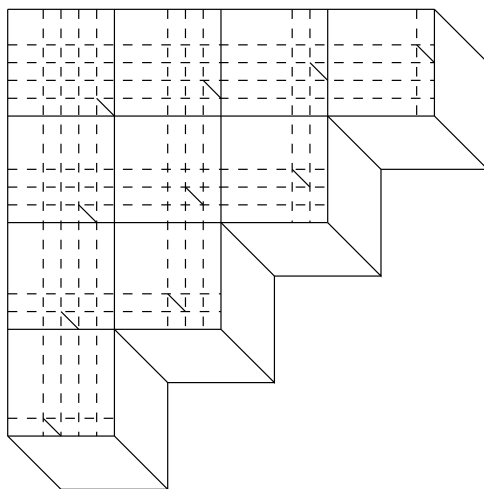
FIG. 3b. \mu = (2^{m_2}, 1^{m_1}) , Level 1
