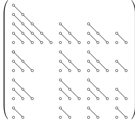
FIG. 1. An element of the centralizer
