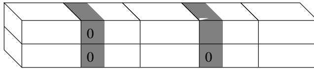
FIG. 6b. \mu = (3, 2) , Level 2
