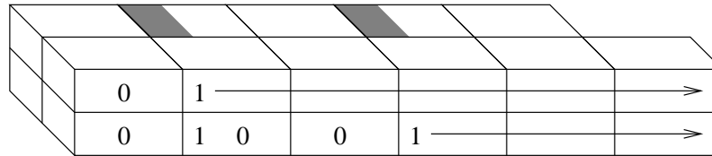
FIG. 6b. \mu = (3, 2) , Level 1
