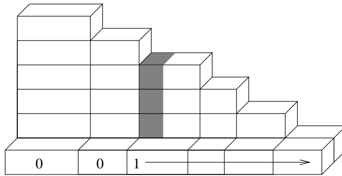
FIG. 5. \mu = (r, 1)
