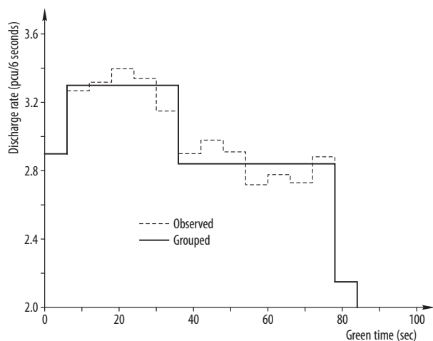
Fig. 6. Discharge rate for site n°4 per 6-second interval
