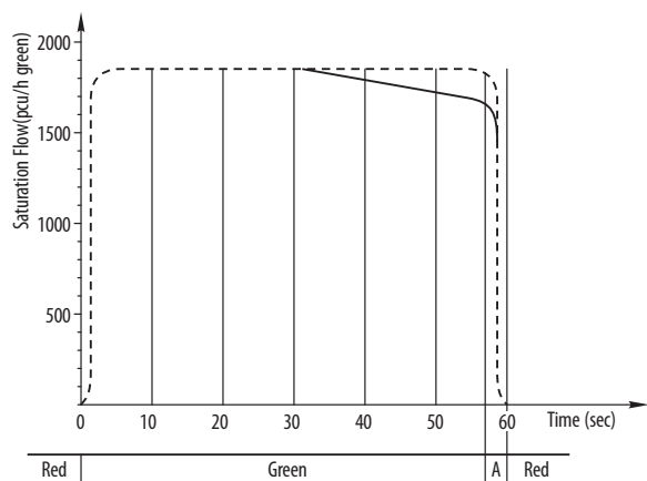
Fig. 2. The concept of saturation flow (Teply et al. 1985)
