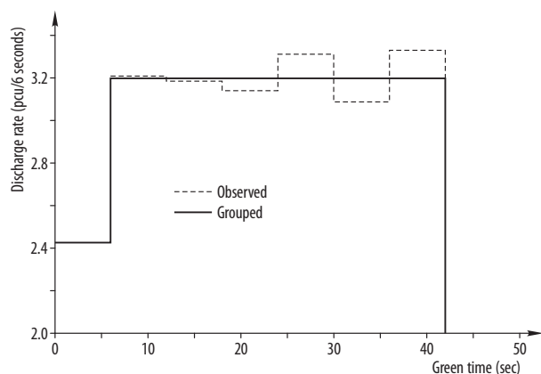
Fig. 4. Discharge rate for site n°2 per 6-second interval
