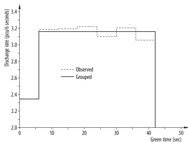
Fig. 5. Discharge rate for site n°3 per 6-second interval
