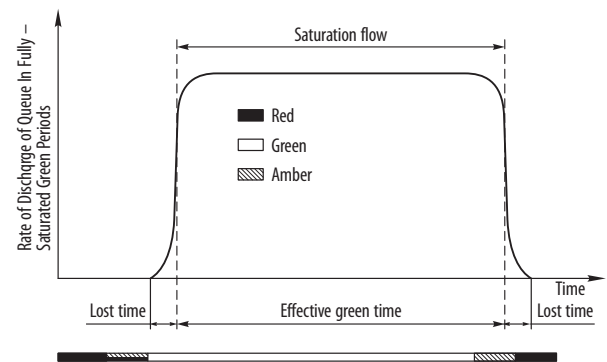
Fig. 1. An idealised model of saturation flow
