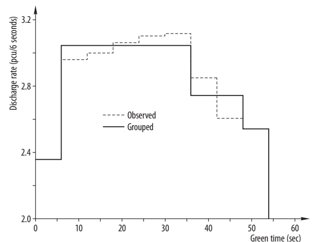
Fig. 3. Discharge rate for site n°1 per 6-second interval
