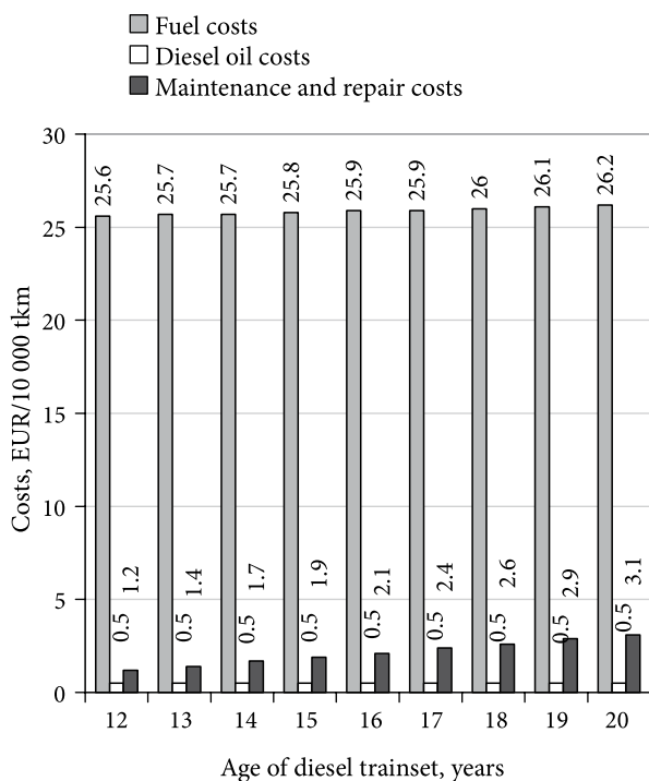
Fig. 2. The relationship between average expenses of diesel train set per 10 000 tkm and its age
